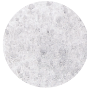
Boric acid
